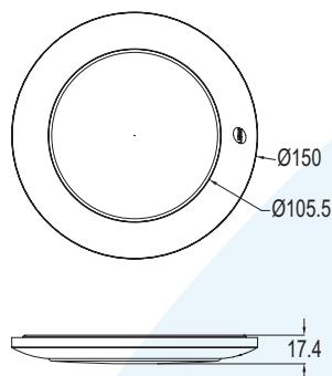
LED 75 CeilingLite touch
